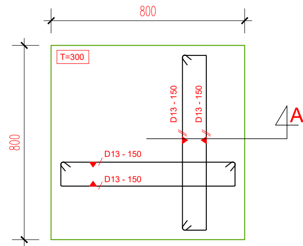
FOOTPLAT FP1
